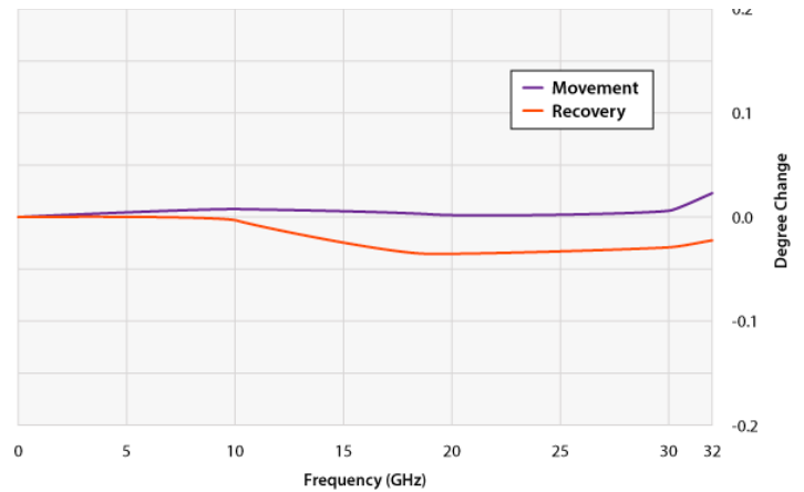
Insertion Loss vs. Flexure
