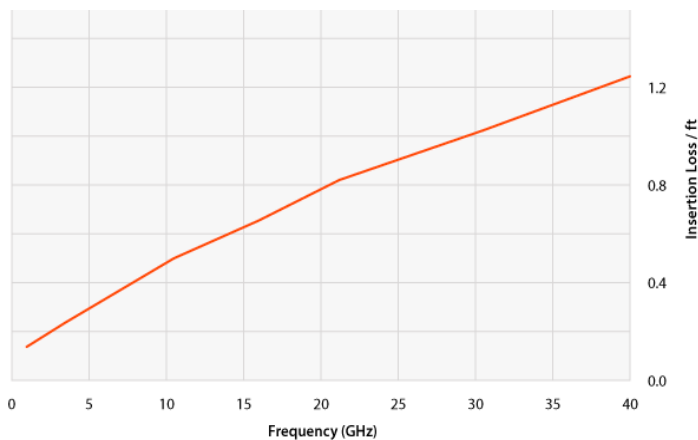
Insertion Loss
