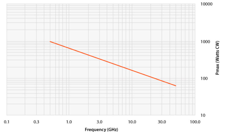
Cable CW Power Handling
