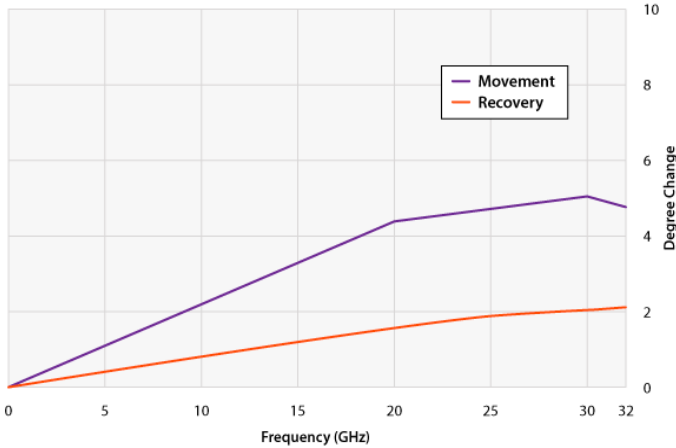
Phase Change vs. Flexure
