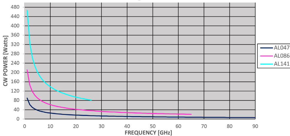
AlumiBend, CW Power Capability 25°C @ Sea Level
